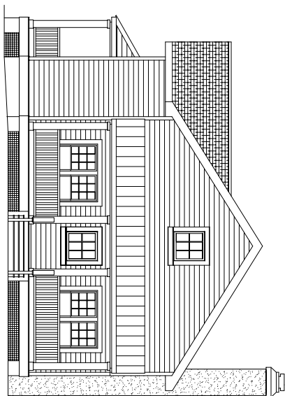
Front Elevation
